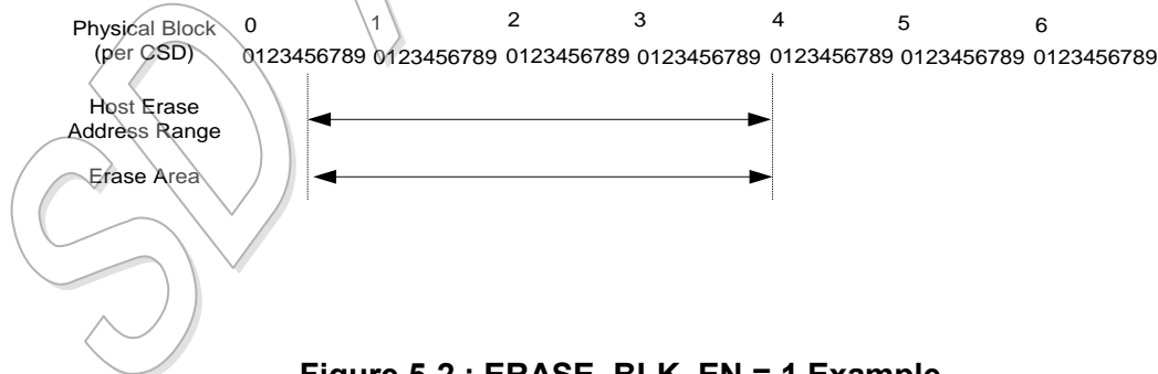
Figure 5-2 : ERASE_BLK_EN = 1 Example
