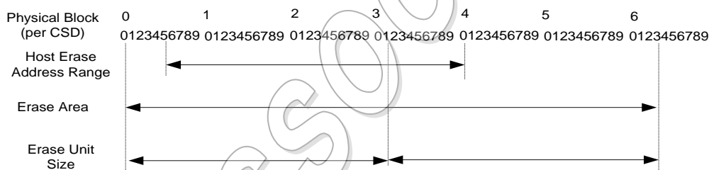
Figure 5-1 : ERASE_BLK_EN = 0 Example
