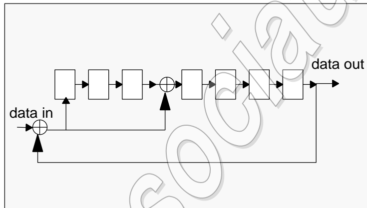
Figure 4-20 : CRC7 Generator/Checker
